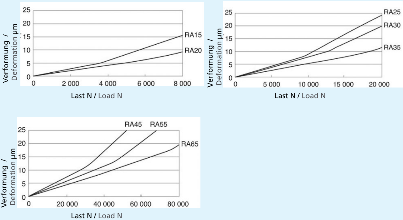
Steifigkeit in vertikaler Richtung (langer Wagen) BN, BL, GM Vertical direction rigidity (Super-High-load type) BN, BL, GM
